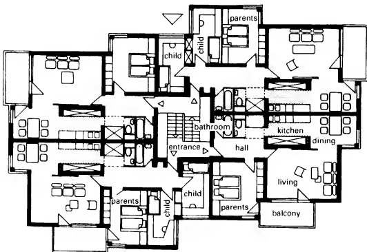
8 Four dwellings per floor: two two-room apartments, two four-room apartments
